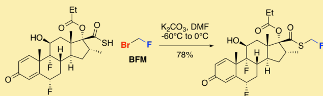
Figure 1. Synthesis of Fluticasone Propionate by Glaxo ( J. Med. Chem. 1994 , 37 , 3717-3729).
